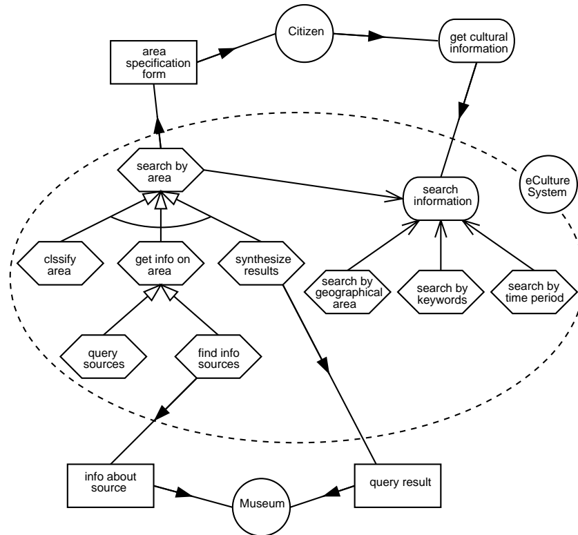
Figure 5. Goal diagram for the goal get cultural information and dependencies between the actor eCulture System and other environment' actors.
