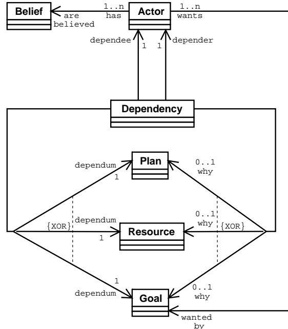
Figure 13. The UML class diagram specifying the actor concept in the Tropos metamodel.
