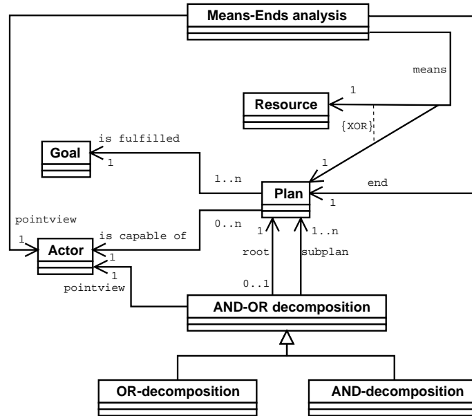
Figure 15. The UML class diagram specifying the plan concept in the Tropos metamodel.
