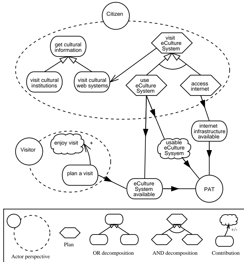
Figure 2. Goal diagrams for Citizen and Visitor. Notice the goal and plan decomposition, the means-end analysis and the (positive)softgoal contribution.
